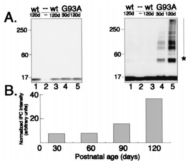
Fig. 5. Accumulation of SOD in IPCs is an early and specific event in spinal cord from mice expressing G93A human SOD. (A) Expression of SOD in transgenic and control mice. Immunoblots of spinal cord extracts (equal \mu\text{g} total protein per lane) from two different mice expressing a wild-type human SOD transgene (lanes 1 and 3), a G93A human SOD transgene at P30 (lane 4) and P120 (lane 5), and from a nontransgenic littermate (lane 2) probed with affinity-purified B1 polyclonal SOD antibody. Blots on Right and Left differ only in the length of time of exposure of the chemiluminescence reaction to film. (B) SOD IPCs increase with age in G93A spinal cords. An immunoblot similar to that in A was probed with affinity-purified B1 antibody. Intensity of high molecular weight, B1-immunoreactive material was quantified from a digital scan of the blot by integrating the total pixel density after subtraction of background intensity from a nontransgenic control lane.
