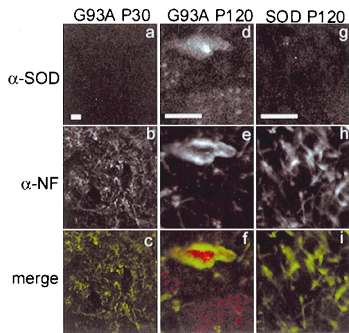
Fig. 4. Inclusion bodies in spinal cords from G93A transgenic mice. Abnormal neurofilament deposition around SOD inclusions in spinal cord motoneurons in G93A transgenic mice at P120 ( d–f ) but not at P30 ( a–c ). Morphology of P30 motoneurons is indistinguishable from that of P120 SOD mice ( g–i ) and from nontransgenic mice (not shown). Spinal cord sections from mice expressing human SOD transgenes were double labeled by indirect immunofluorescence using affinity purified polyclonal antibody to SOD ( a , d , and g ) and mAb to phosphorylated neurofilament ( b , e , and h ) and visualized by confocal microscopy. Note magnification in a–d is lower than that in d–i . (Bars = 10 \mu\text{m} .)
